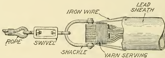
Fig. 49. Tackle for Fastening Cable to Rope to Draw Cable Through Ducts
